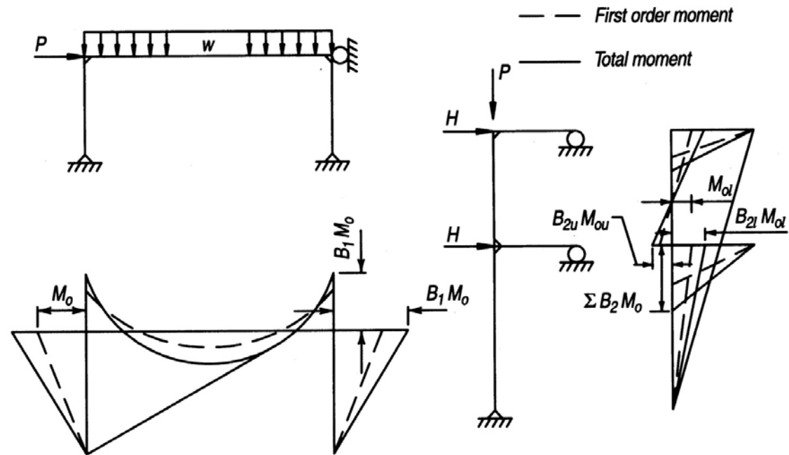
Fig. C-A-8.1. Moment amplification.
