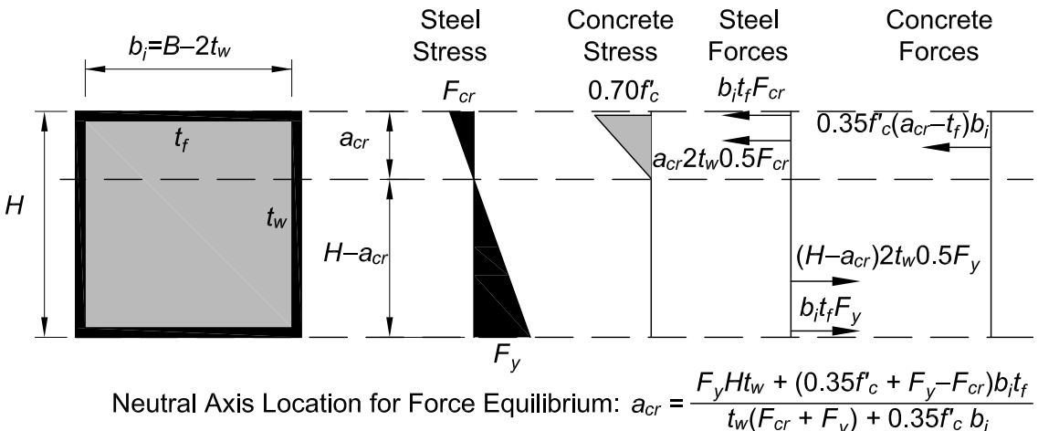
(c) Slender section—stress blocks for calculating first yield moment, M_{cr}
